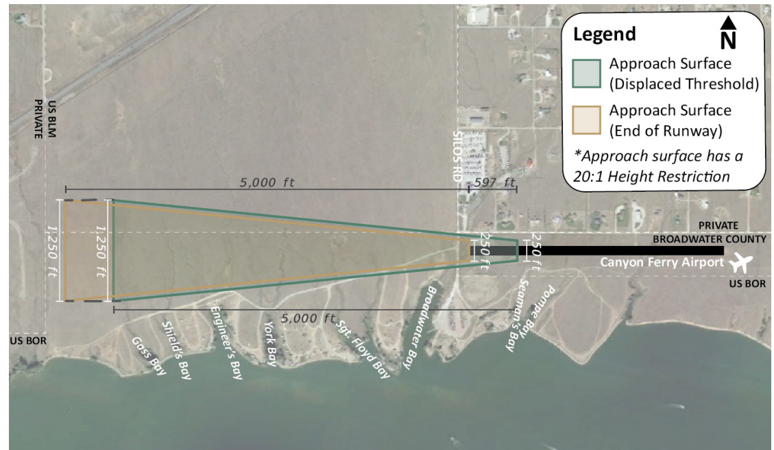
Figure 8: Canyon Ferry Airport Approach Surface
