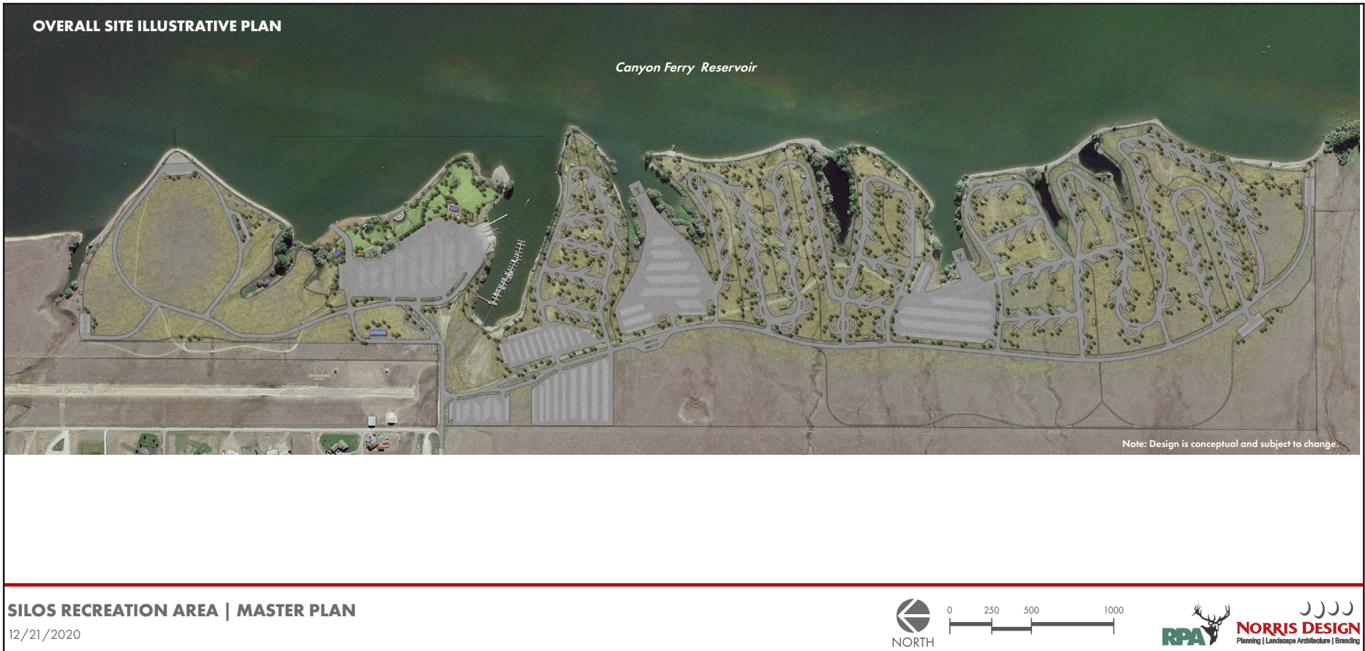
Figure 14: Site Schematic
