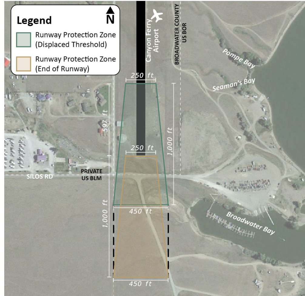
Figure 7: Canyon Ferry Airport RPZ
